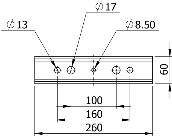
Hole pattern in mounting bracket
