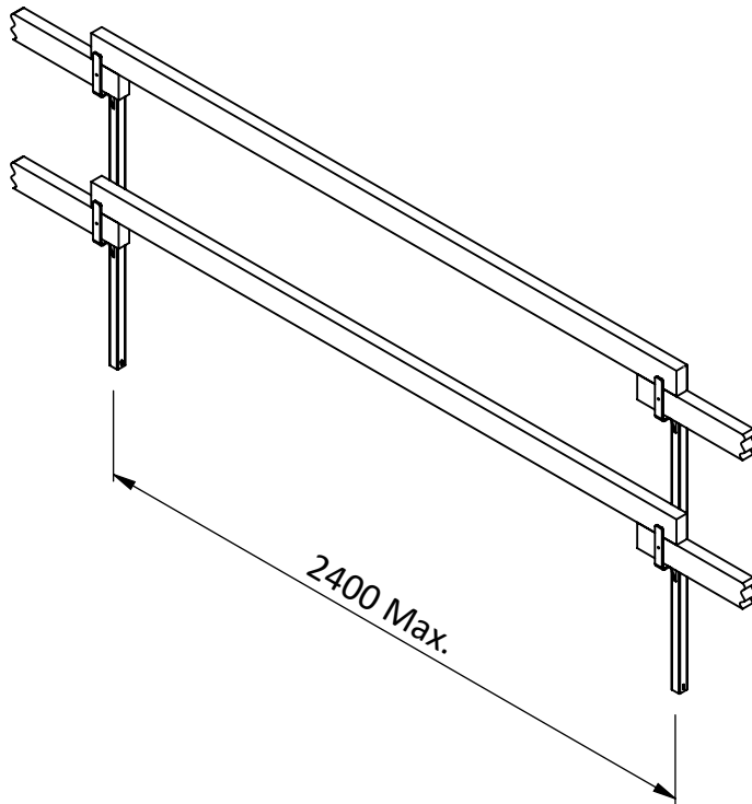
45 x 95mm Timber Guard Rail NOTE: Class A only
